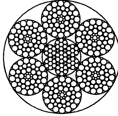
6x49 SWS (16-8+8-8-1) (CWR) 48 to 92 mm
