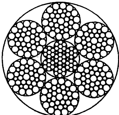
6x36 SW (14-7+7-7-1) (CWR) 13 to 56 mm
