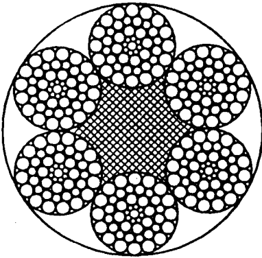
6x41 SW (16-8+8-8-1) (CF) 16 to 60 mm
