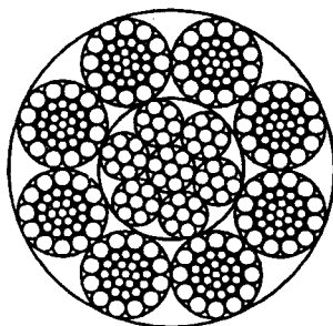
8x37 SF (12-12-6F-6-1) (CWR)
