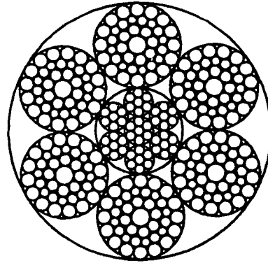
6x41 SW (16-8+8-8-1) (CWR) 16 to 60 mm
