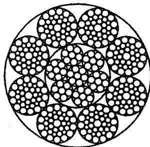
8x36 SW (14-7+7-7-1) (CWR)
