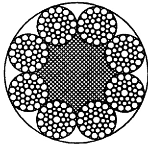
8x36 SW (14-7+7-7-1) (CF)
