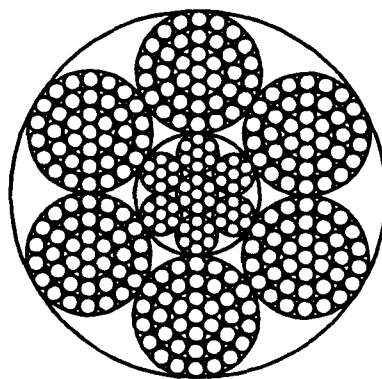
8 to 52 mm With Steel Core (CWR)
