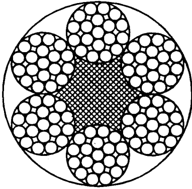
With Fibre Core (CF)
