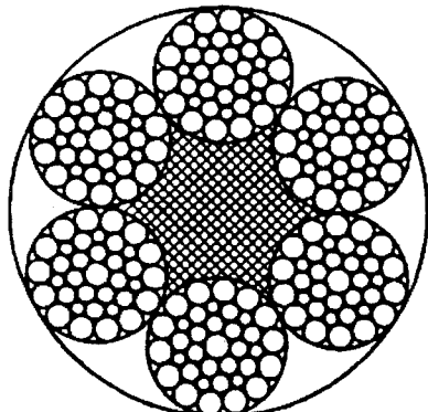
6x36 SW (14-7+7-7-1) (CF) 13 to 56 mm
