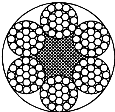
8 to 52 mm With Fibre Core (CF)
