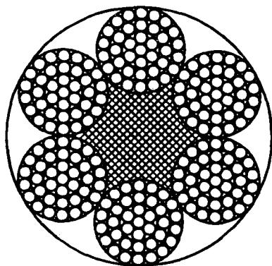
8 to 64 mm With Fibre Core (CF)
